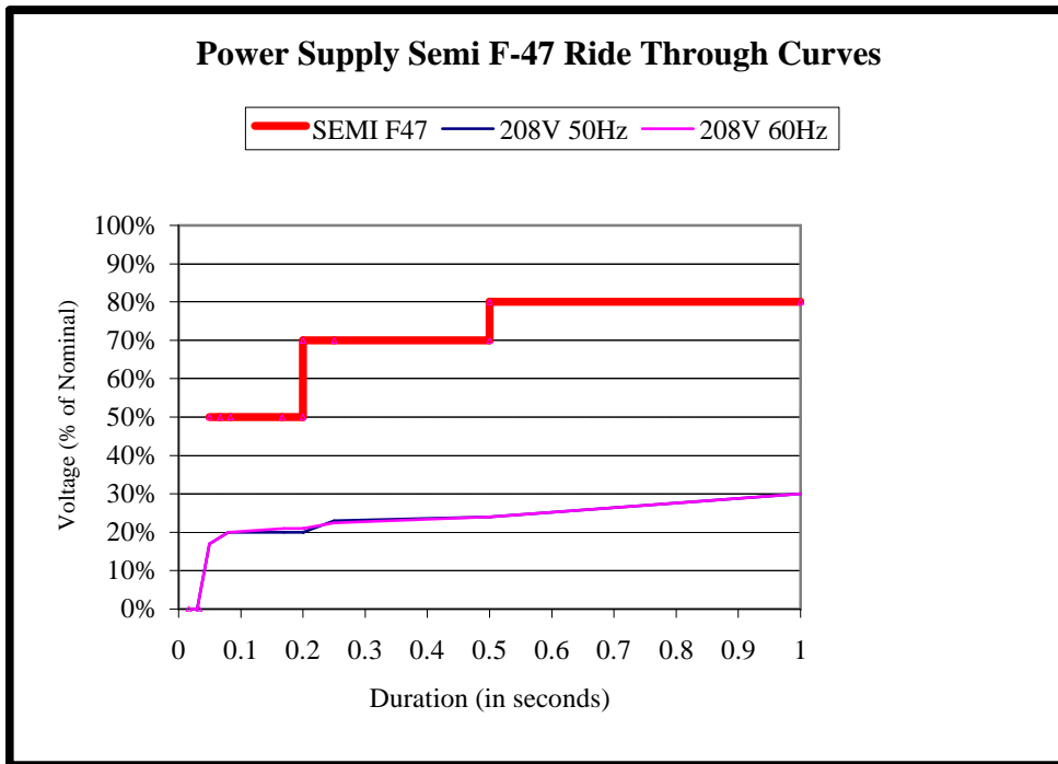
Figure A-2. PULS QS10.DNET SEMI F47 Ride-Through Curve at 208Vac
